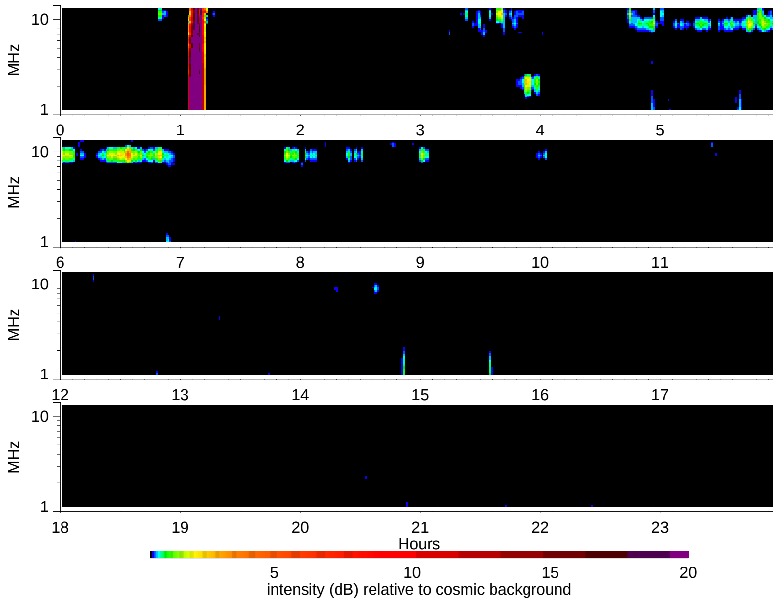
Wind Waves RAD2 receiver: 1995/1/1
