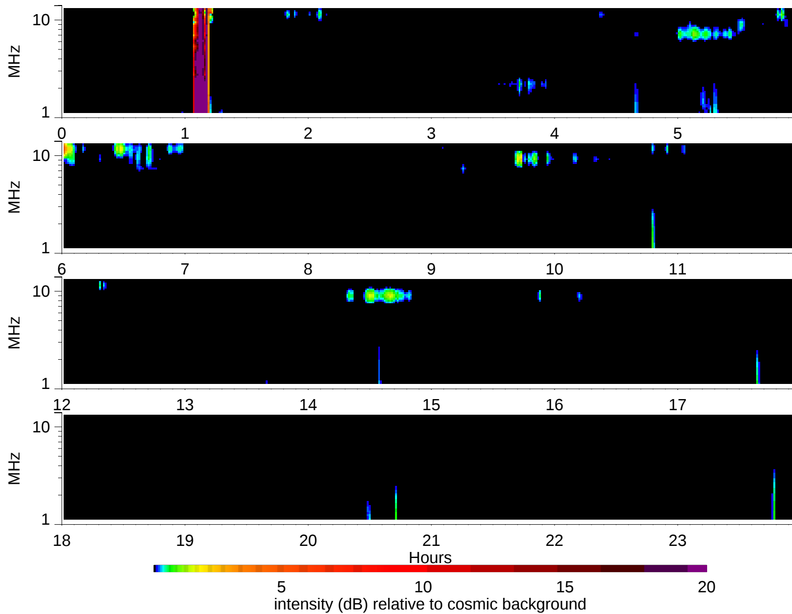
Wind Waves RAD2 receiver: 1995/1/2
