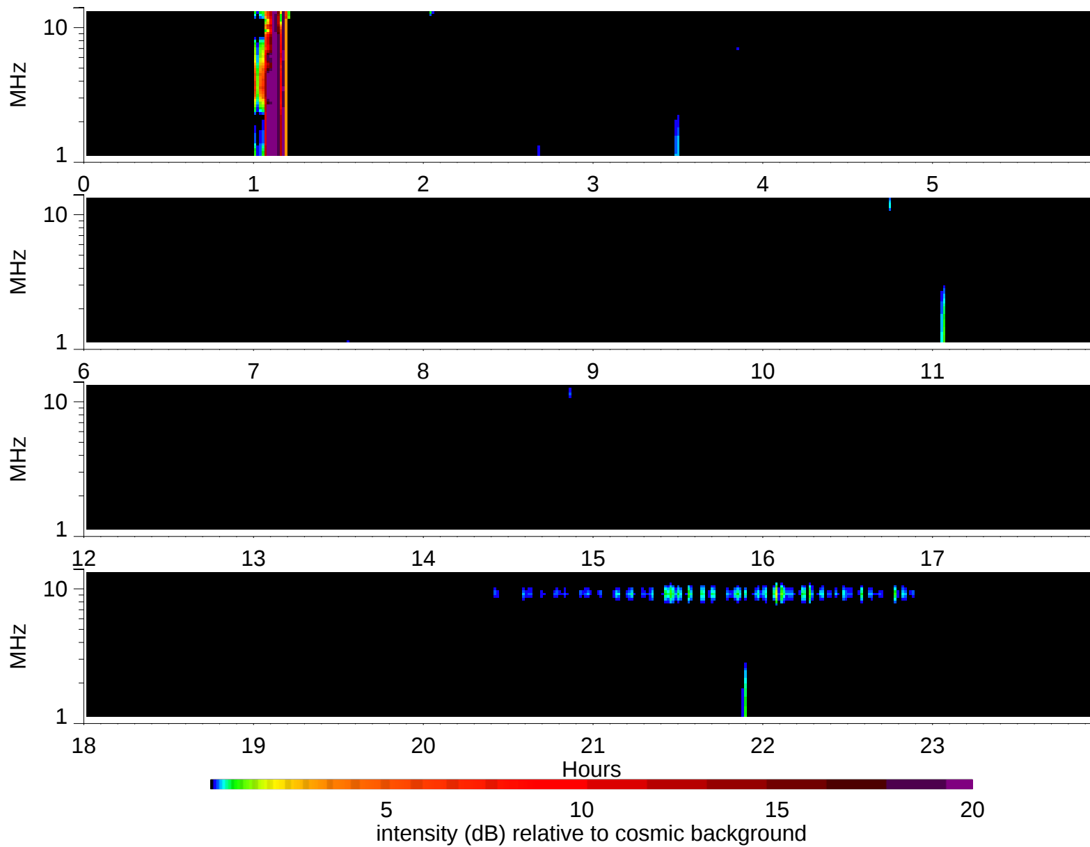
Wind Waves RAD2 receiver: 1995/1/7
