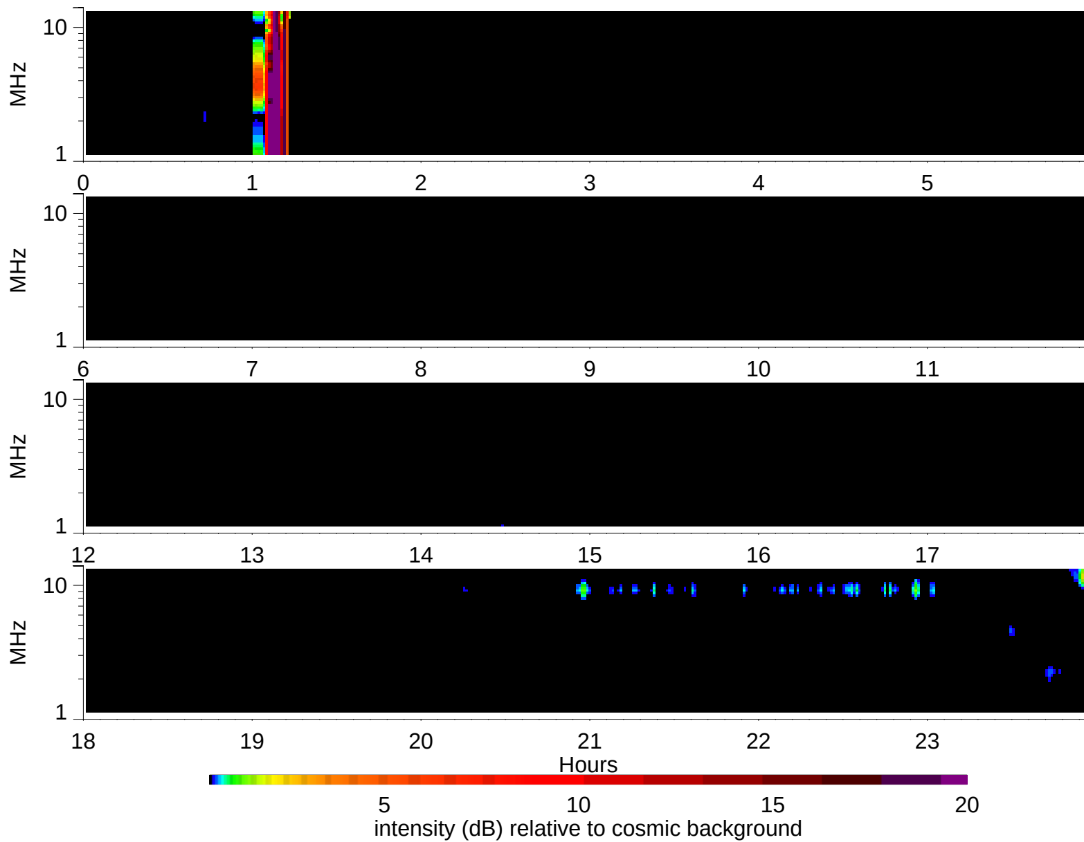
Wind Waves RAD2 receiver: 1995/1/10
