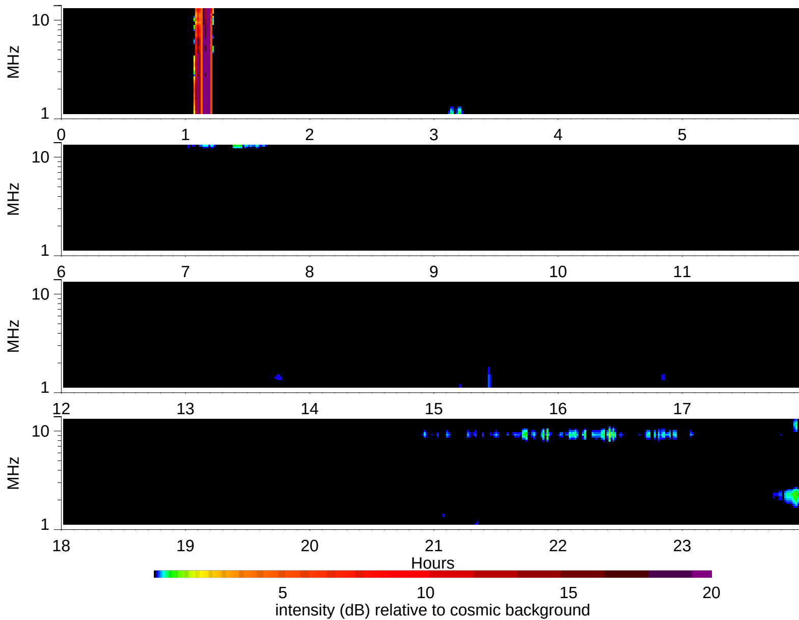
Wind Waves RAD2 receiver: 1995/1/11
