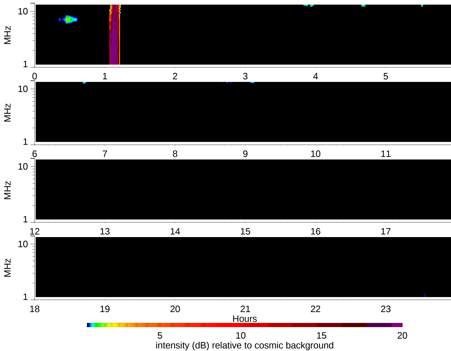
Wind Waves RAD2 receiver: 1995/1/12
