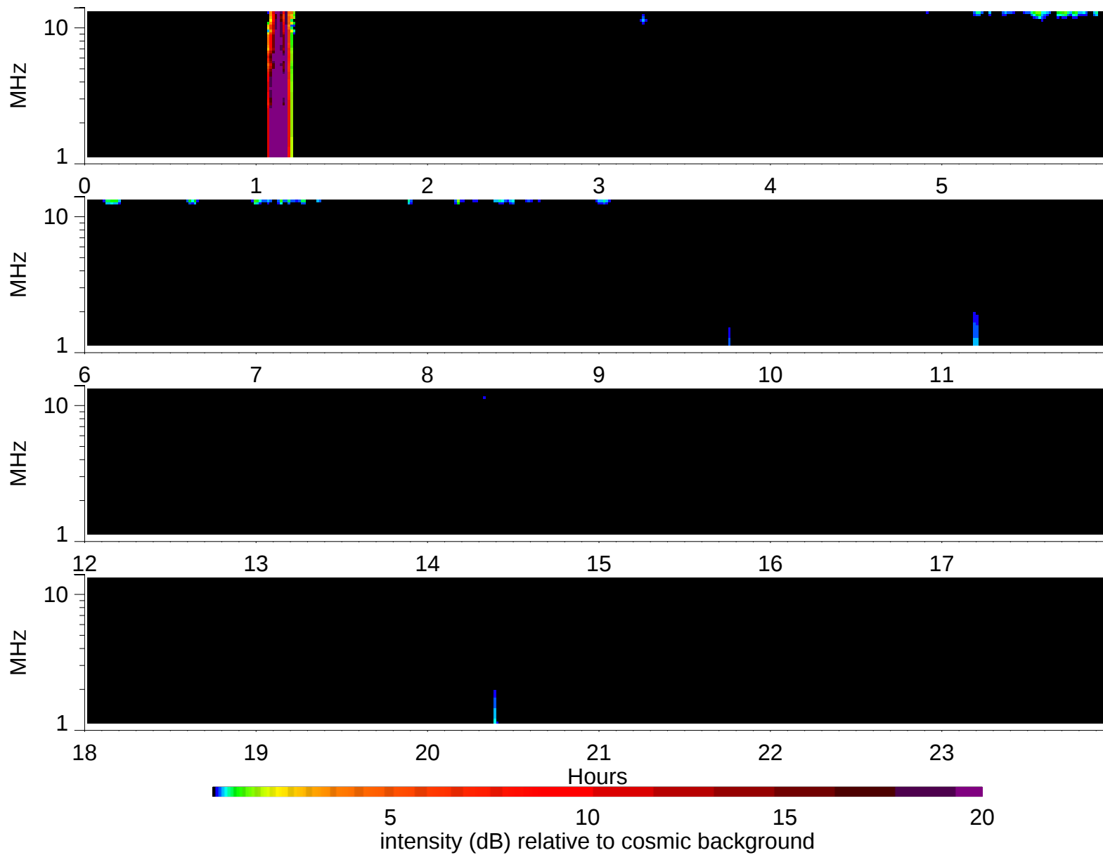
Wind Waves RAD2 receiver: 1995/1/13
