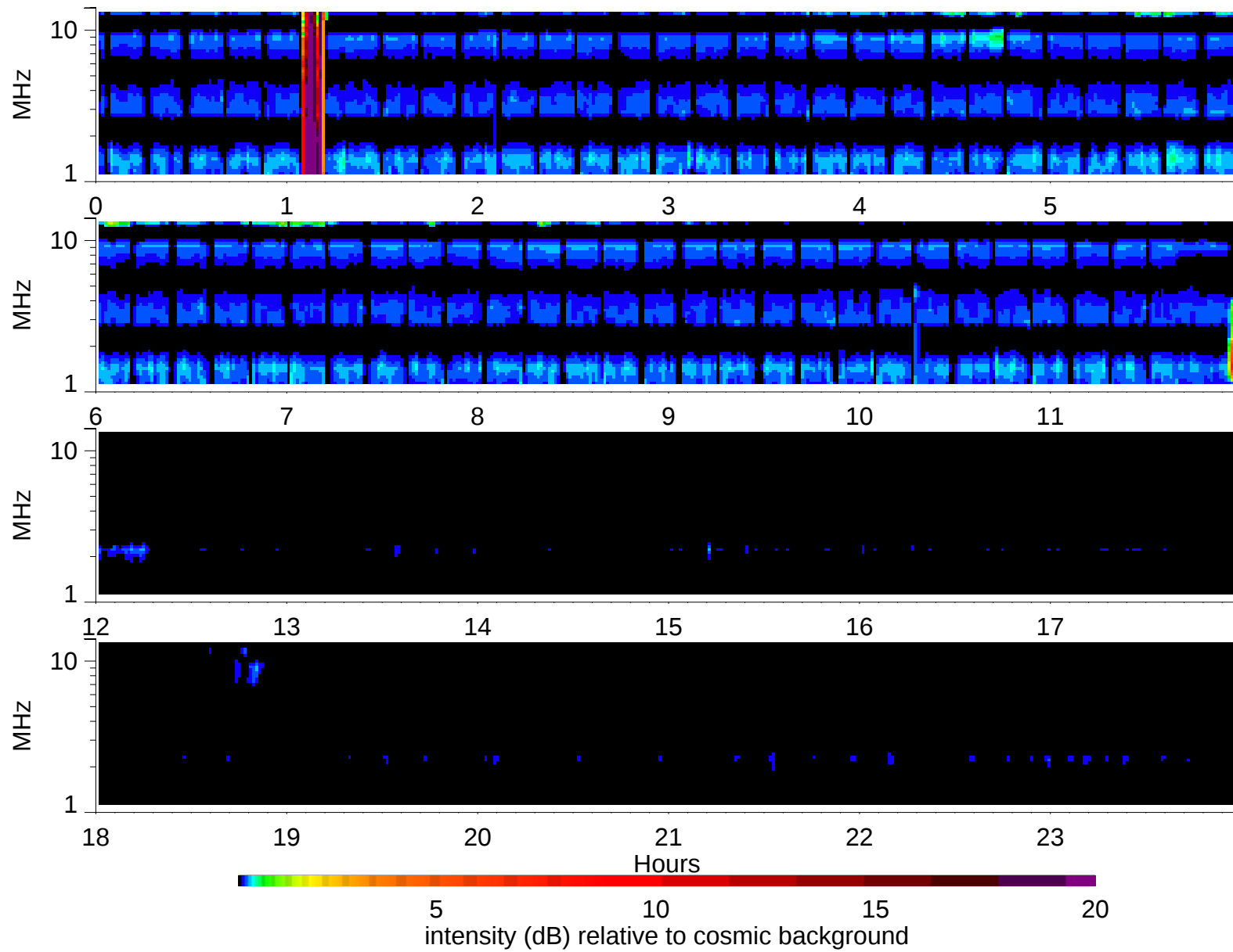
Wind Waves RAD2 receiver: 1995/1/14
