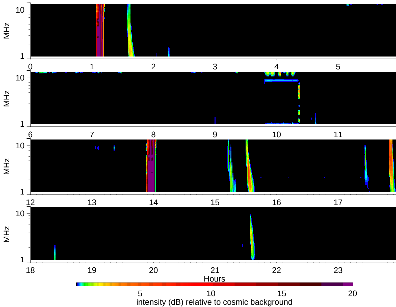
Wind Waves RAD2 receiver: 1995/1/15
