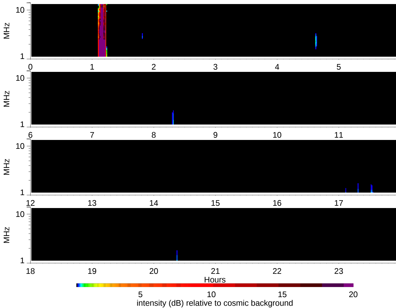
Wind Waves RAD2 receiver: 1995/1/22
