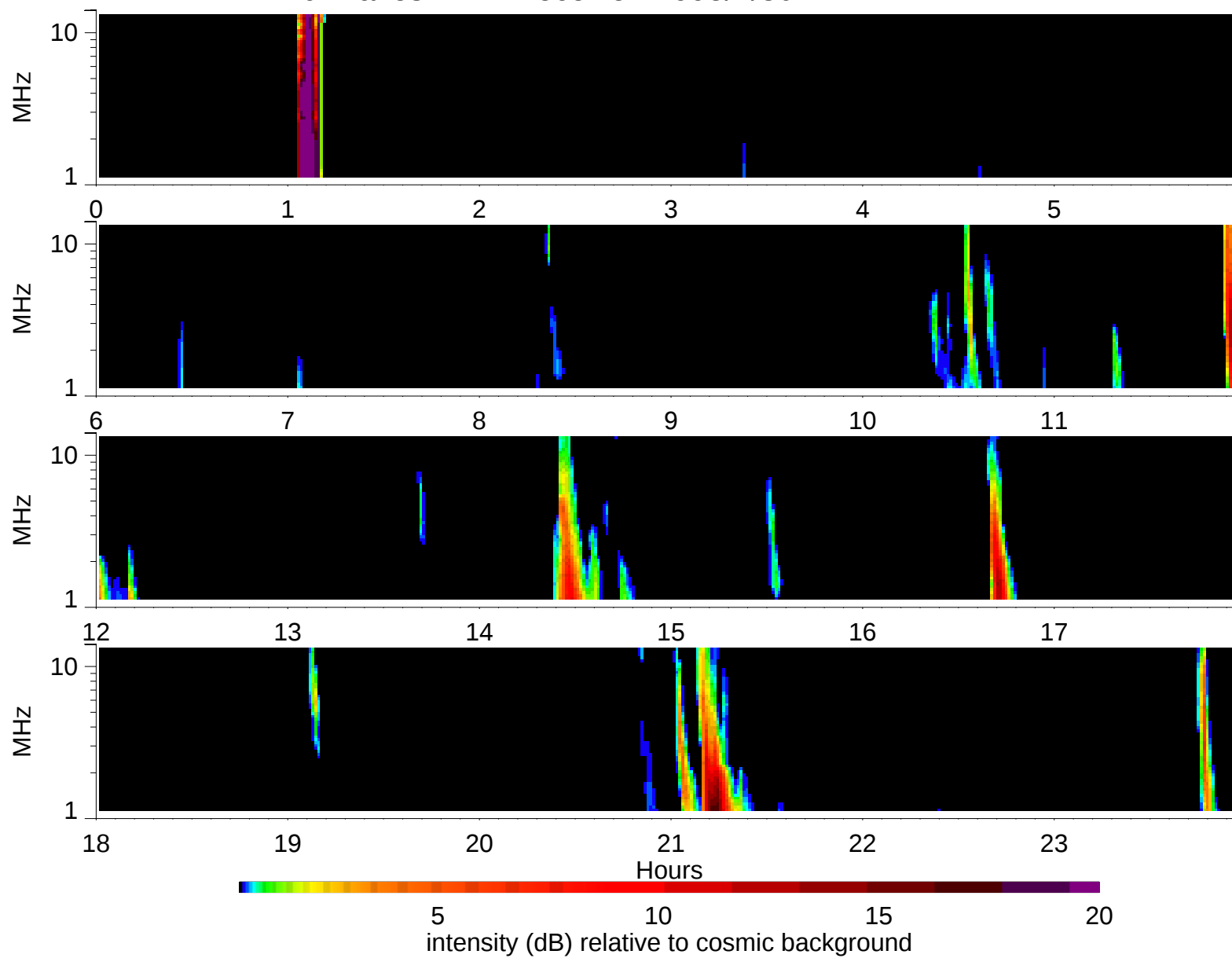
Wind Waves RAD2 receiver: 1995/1/30
