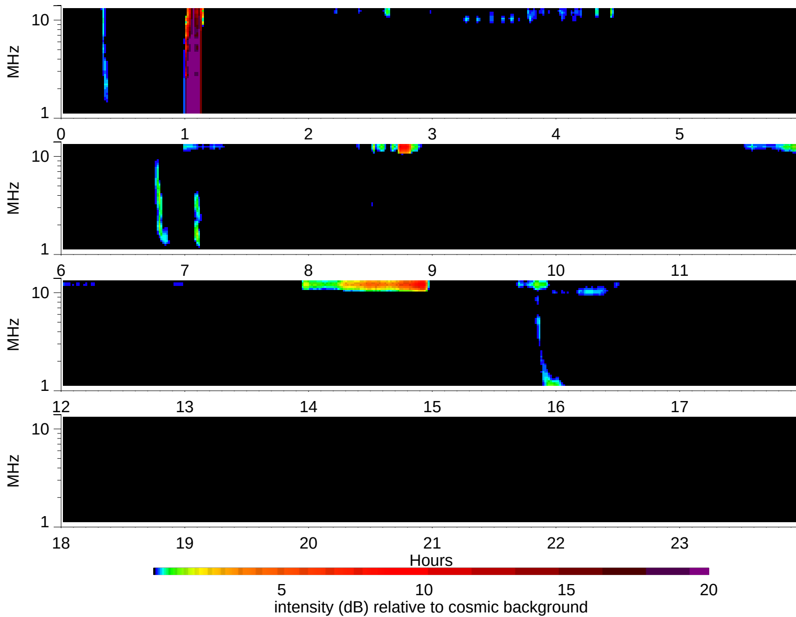
Wind Waves RAD2 receiver: 1995/2/4
