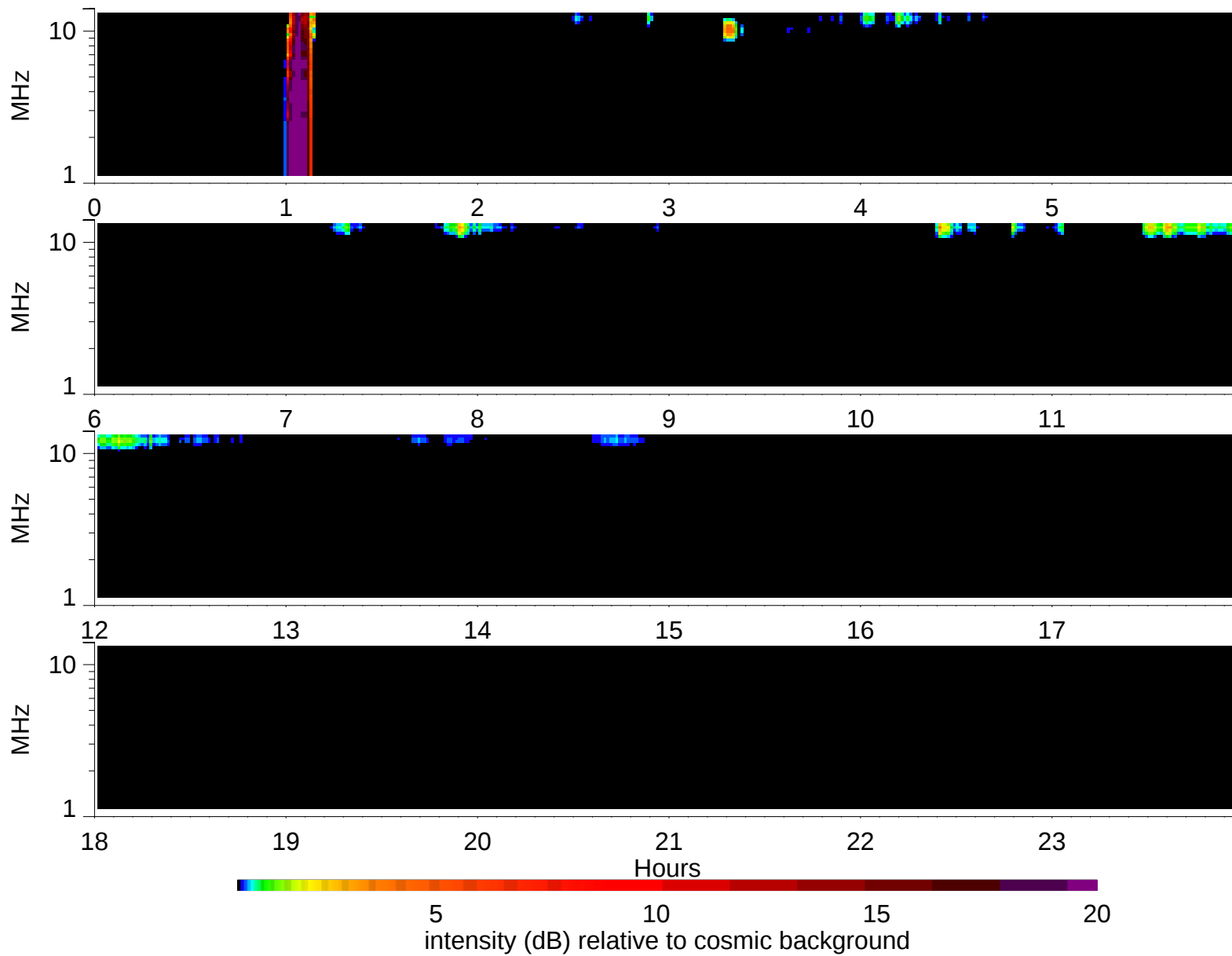
Wind Waves RAD2 receiver: 1995/2/5
