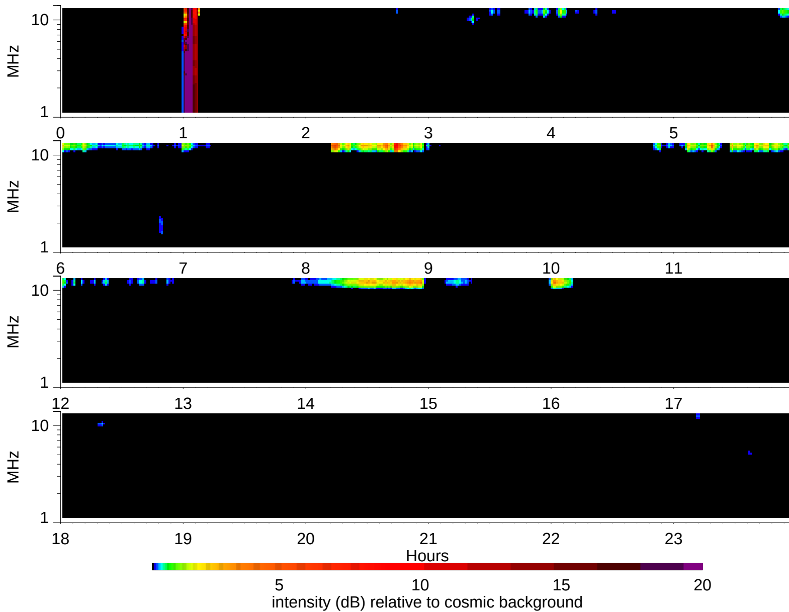
Wind Waves RAD2 receiver: 1995/2/7
