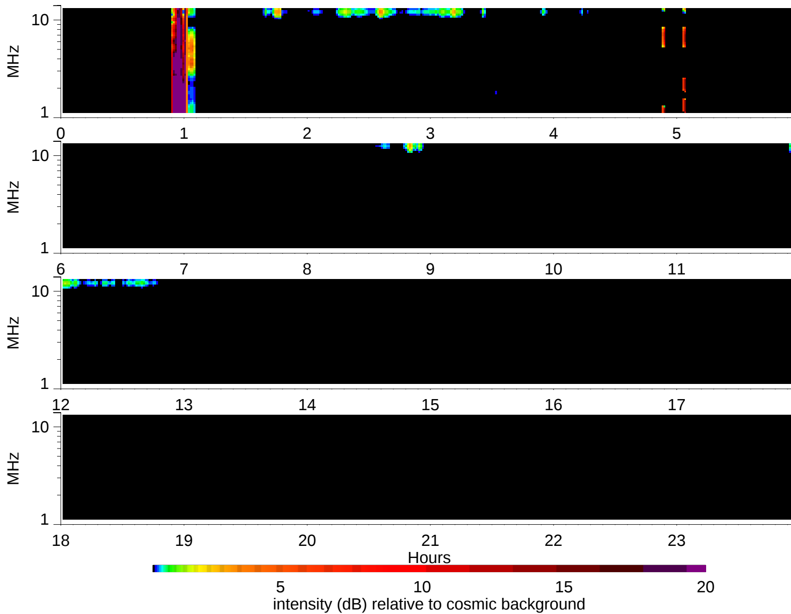
Wind Waves RAD2 receiver: 1995/2/21
