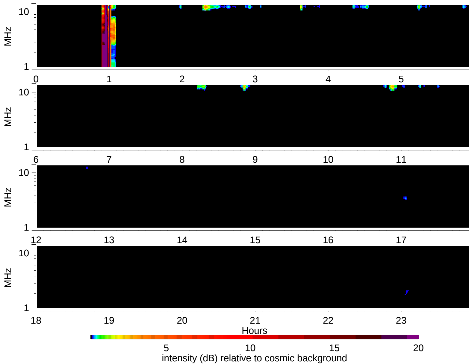
Wind Waves RAD2 receiver: 1995/2/22
