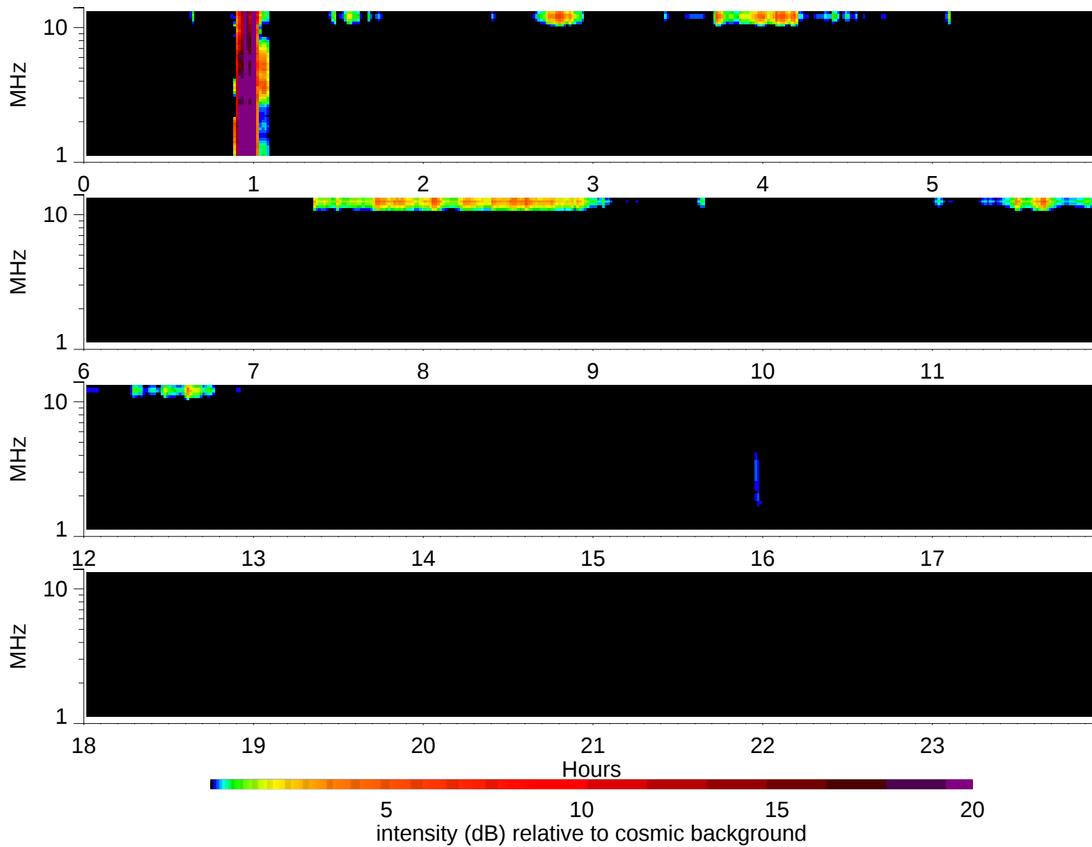
Wind Waves RAD2 receiver: 1995/2/23
