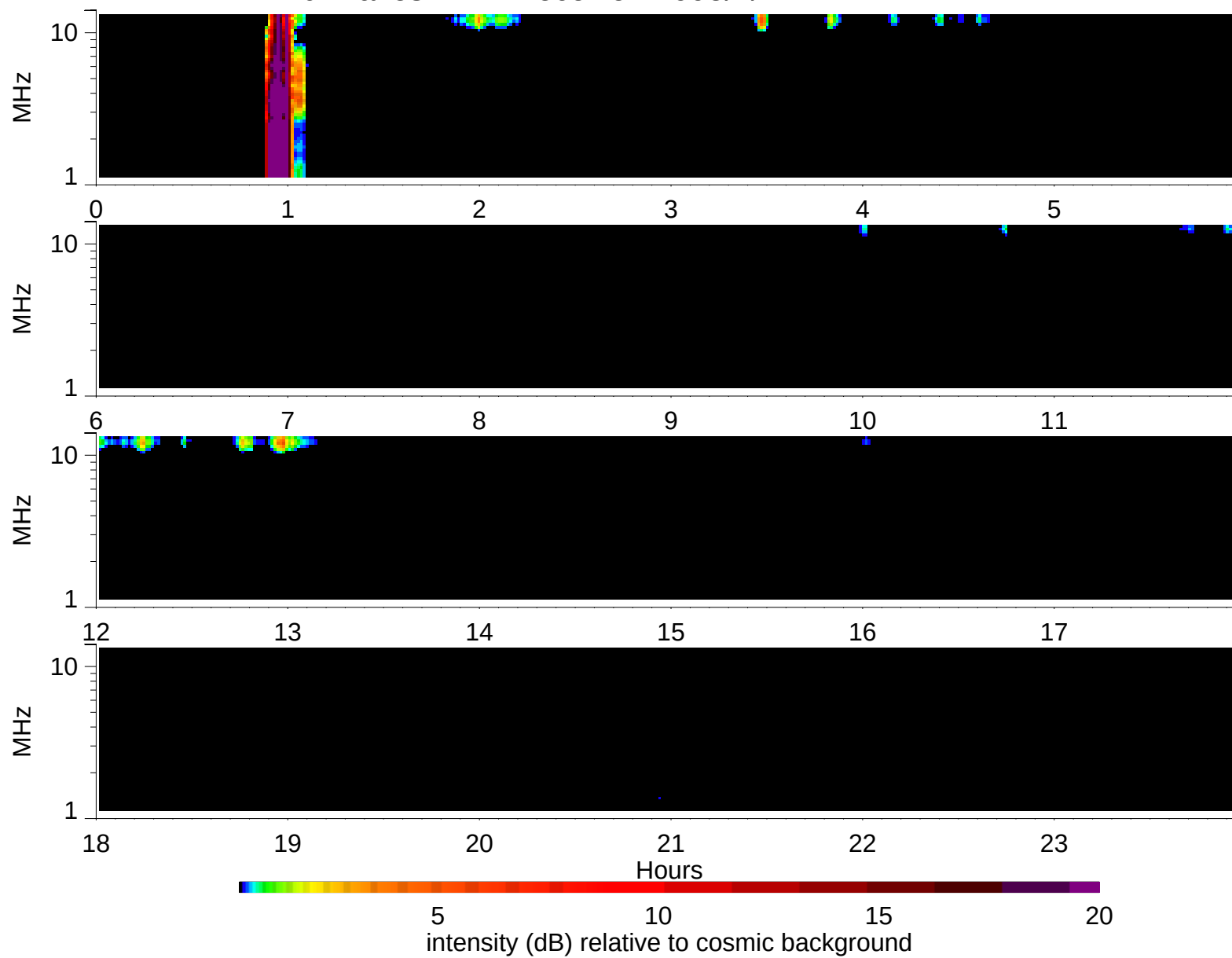
Wind Waves RAD2 receiver: 1995/2/24
