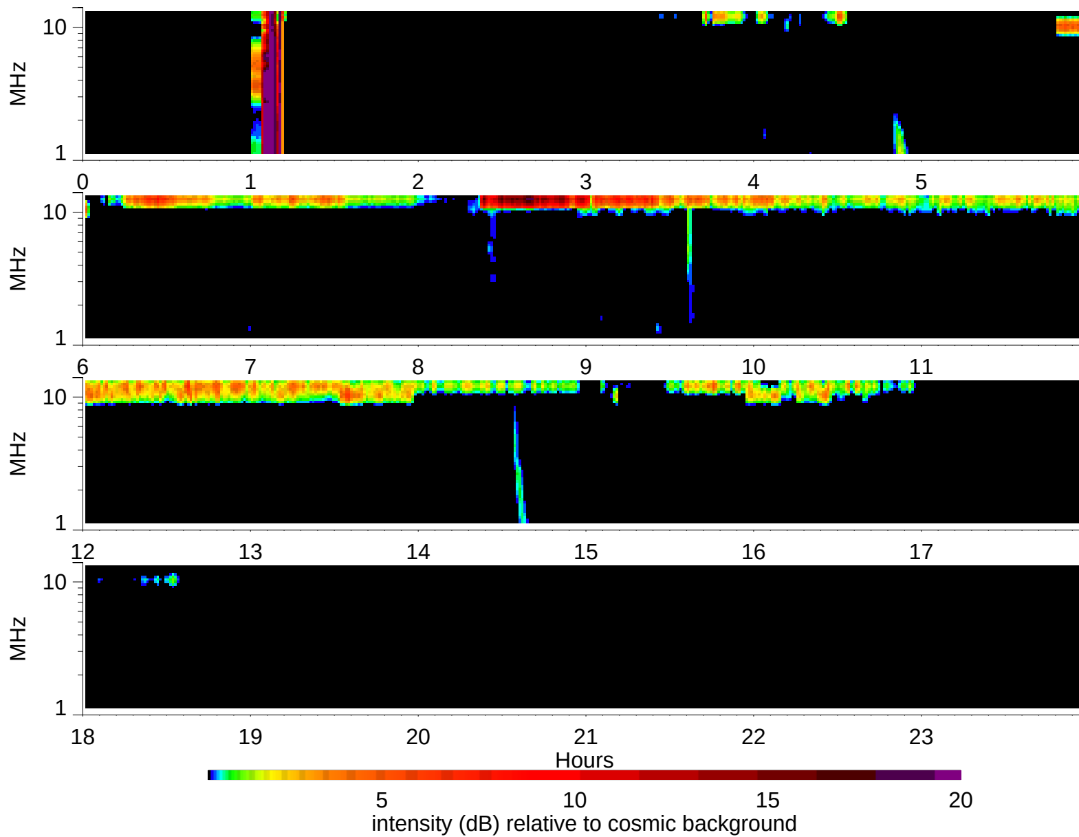
Wind Waves RAD2 receiver: 1995/3/5
