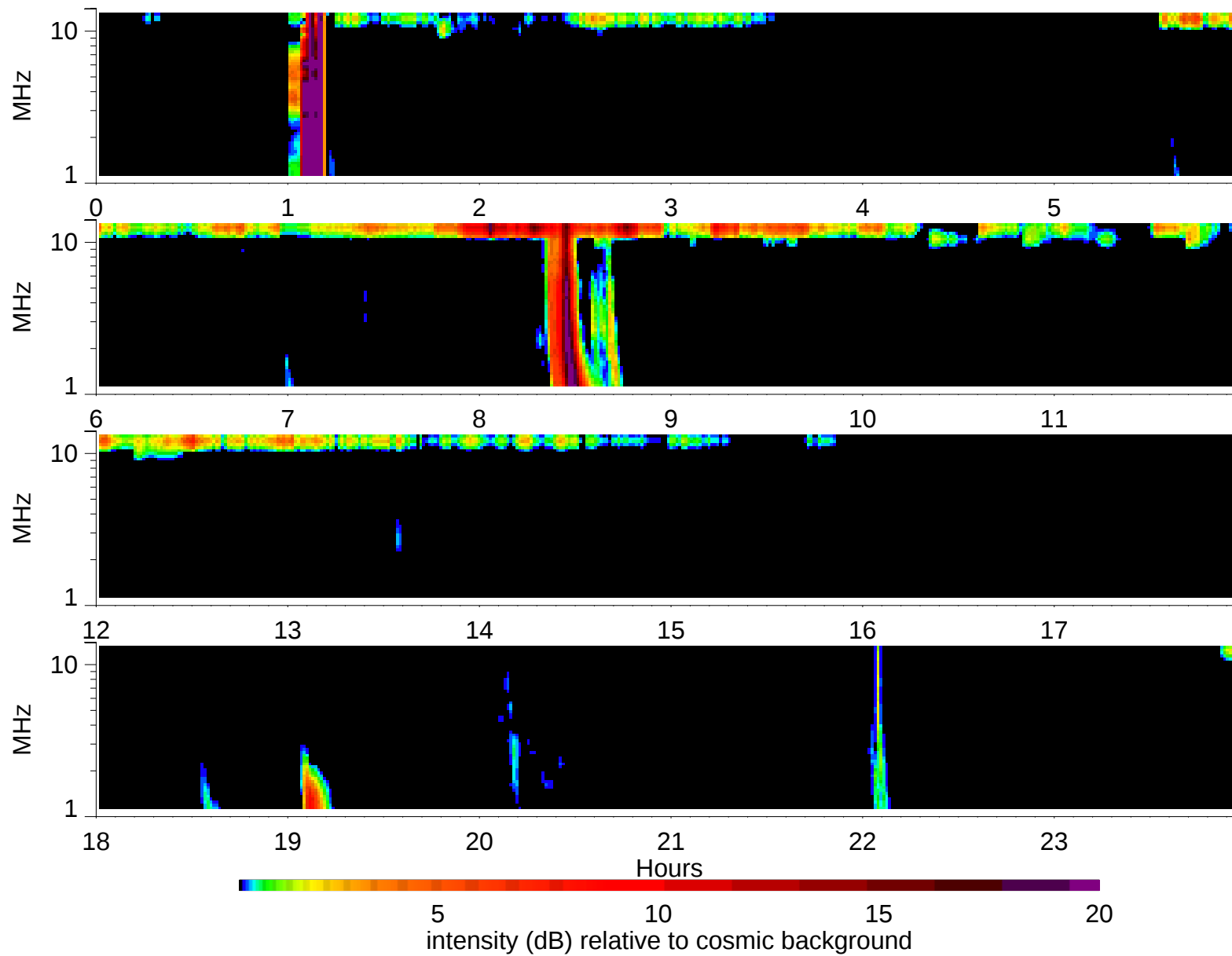
Wind Waves RAD2 receiver: 1995/3/6
