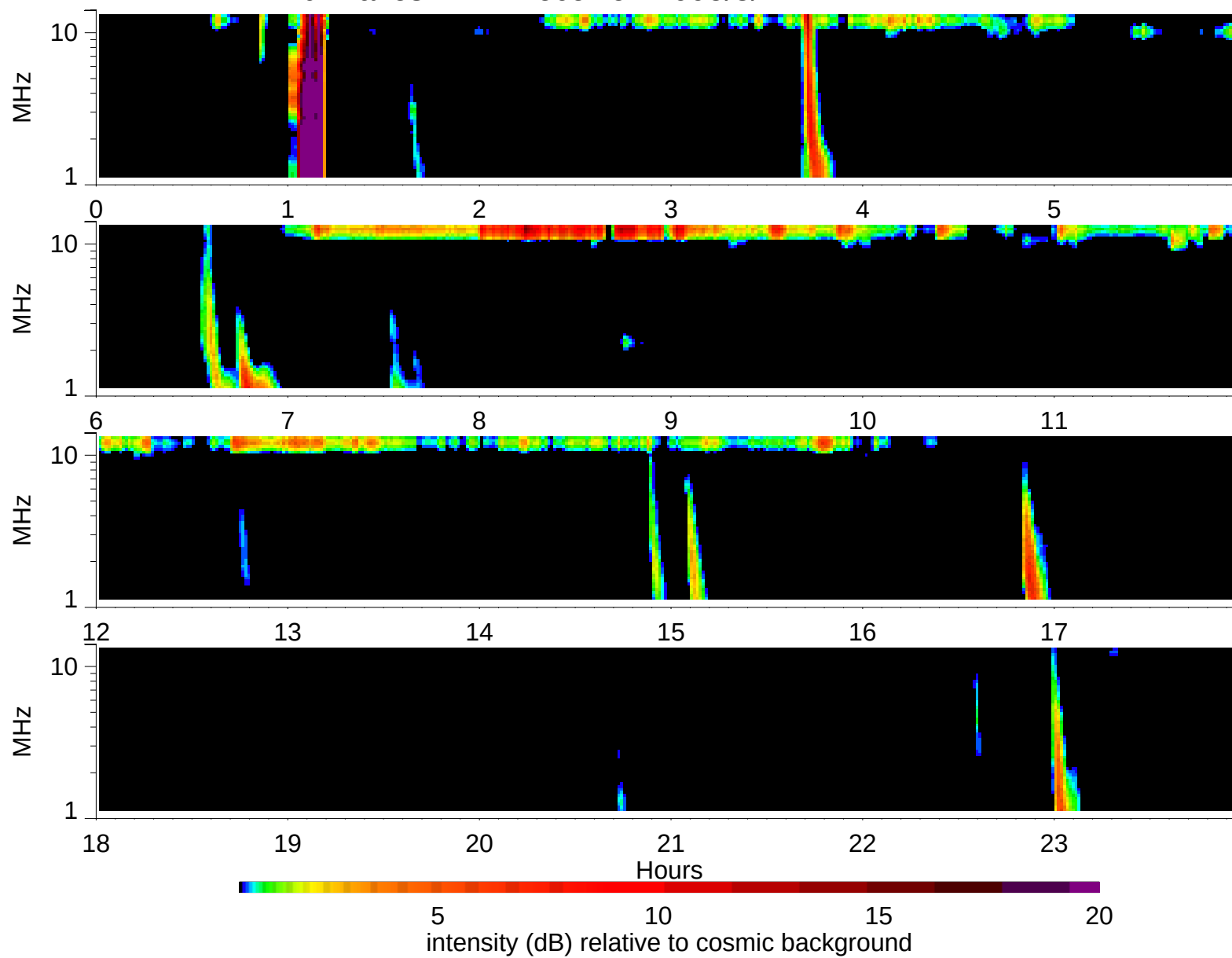
Wind Waves RAD2 receiver: 1995/3/7
