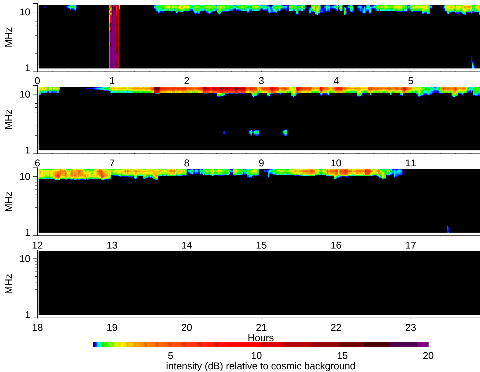
Wind Waves RAD2 receiver: 1995/3/19
