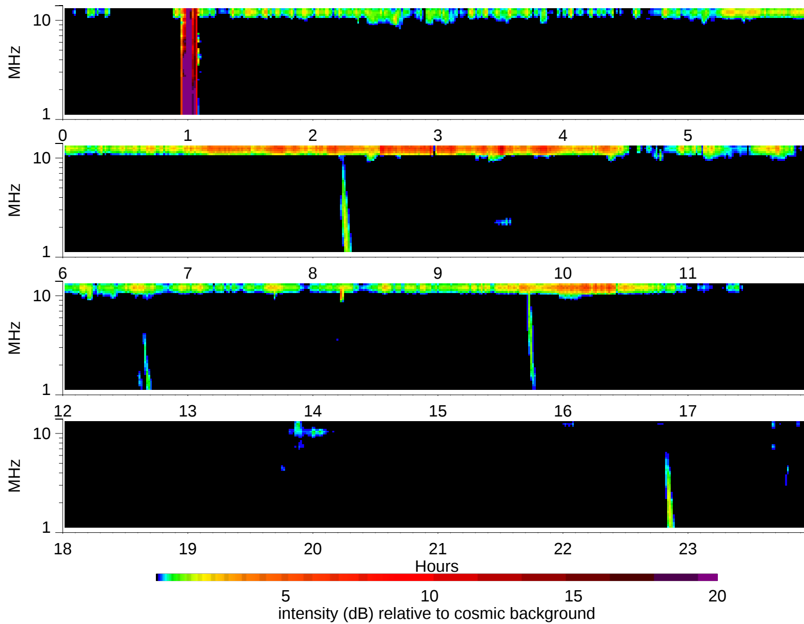
Wind Waves RAD2 receiver: 1995/3/24
