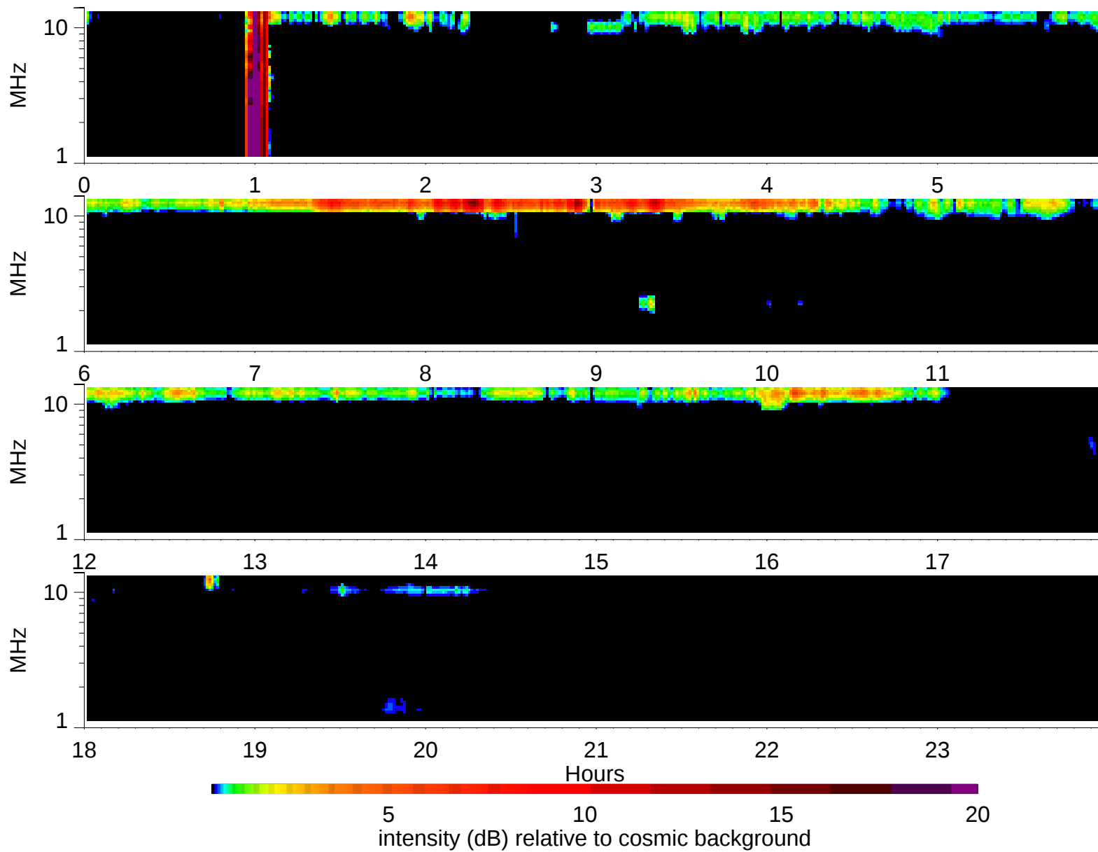
Wind Waves RAD2 receiver: 1995/3/25
