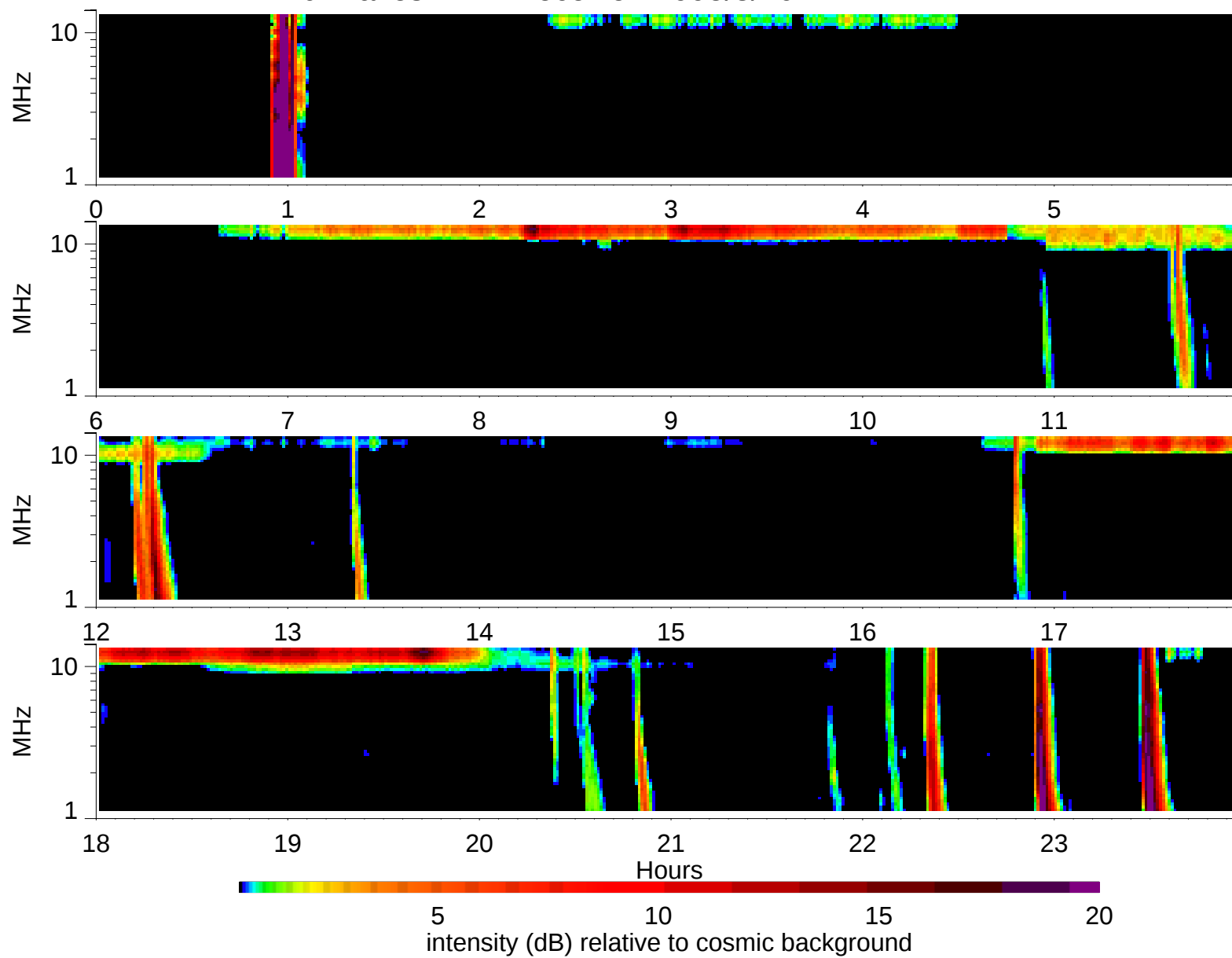
Wind Waves RAD2 receiver: 1995/3/26
