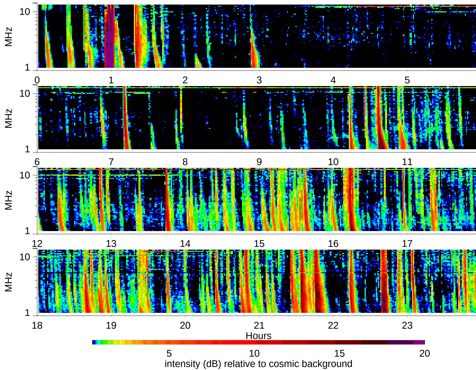
Wind Waves RAD2 receiver: 1995/3/28
