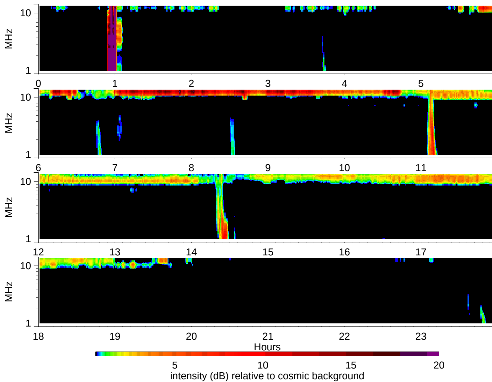
Wind Waves RAD2 receiver: 1995/4/2
