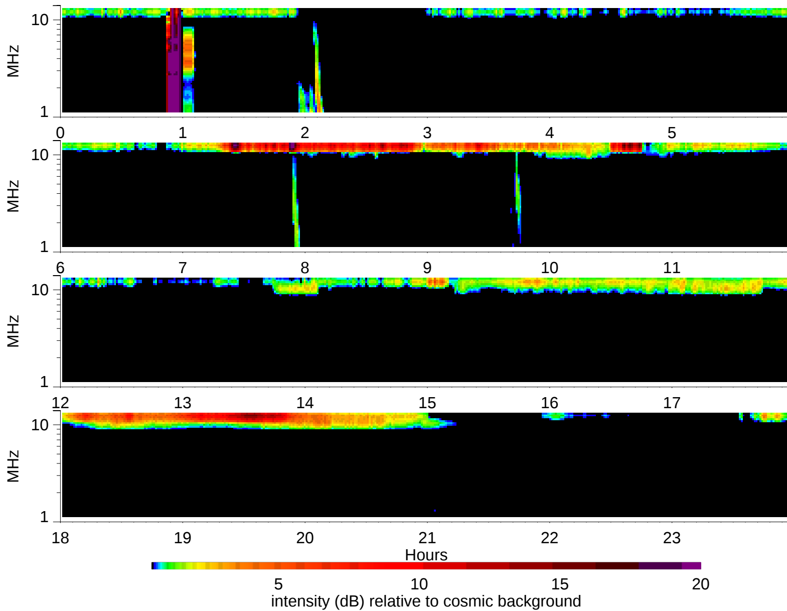
Wind Waves RAD2 receiver: 1995/4/4
