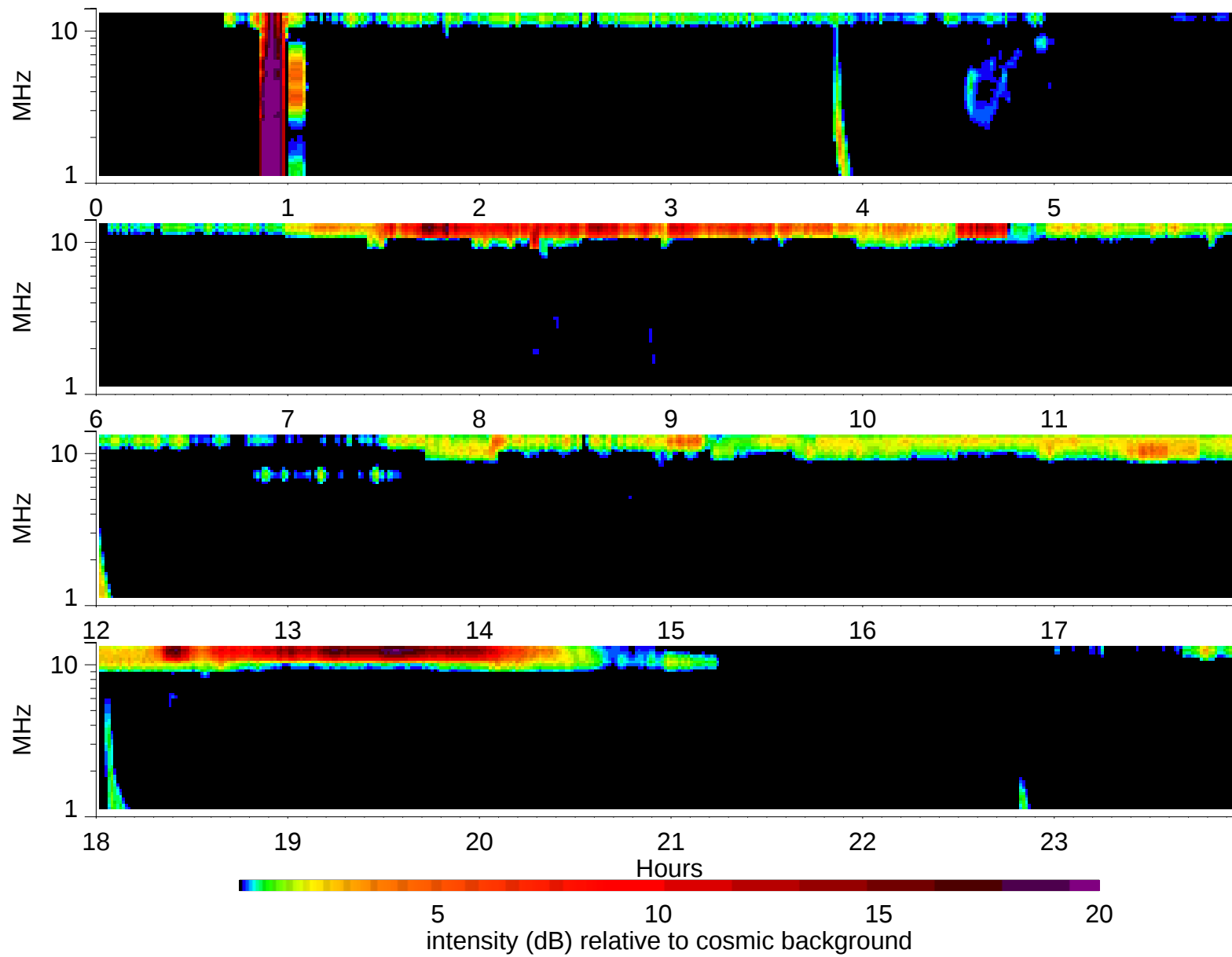
Wind Waves RAD2 receiver: 1995/4/6
