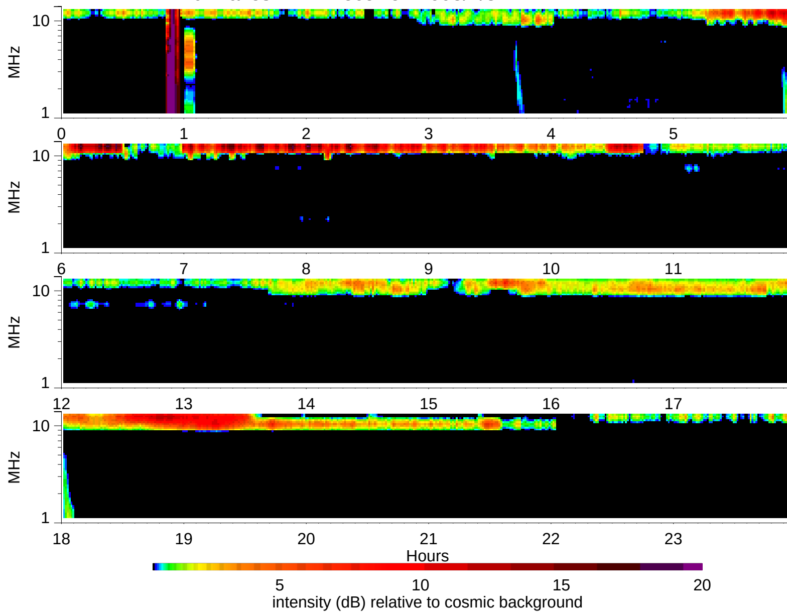
Wind Waves RAD2 receiver: 1995/4/8
