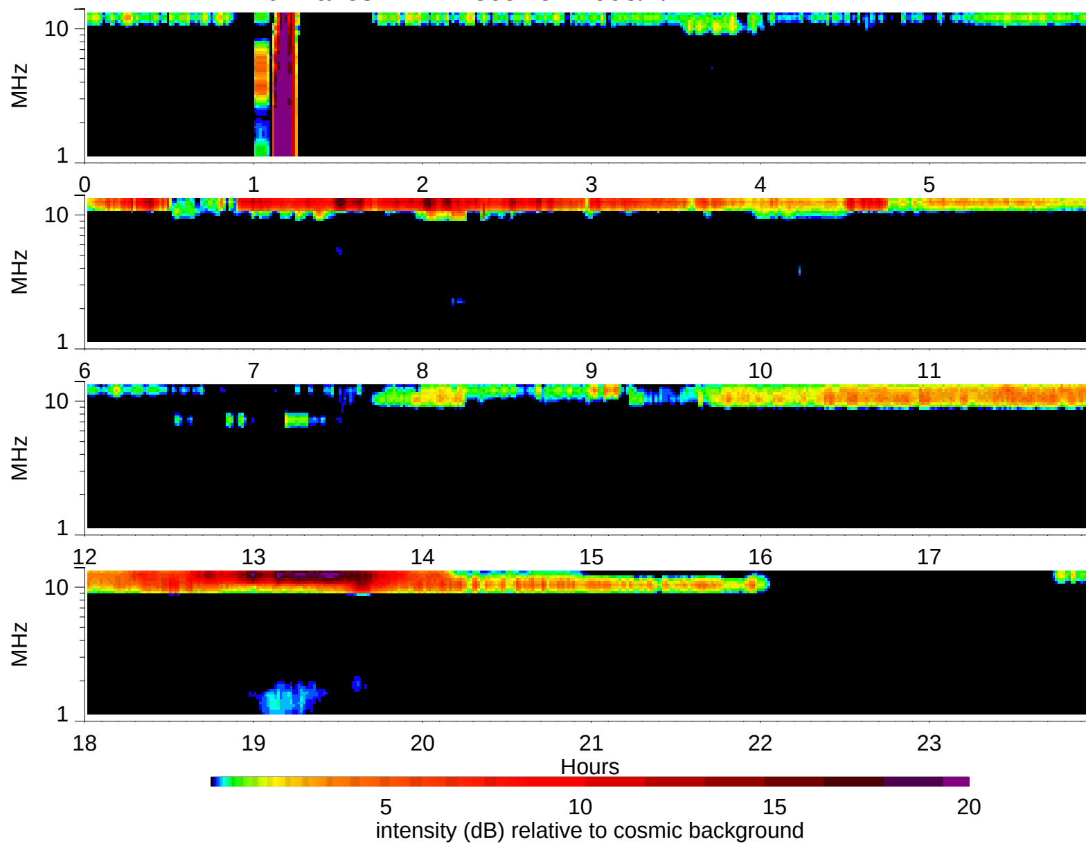
Wind Waves RAD2 receiver: 1995/4/11
