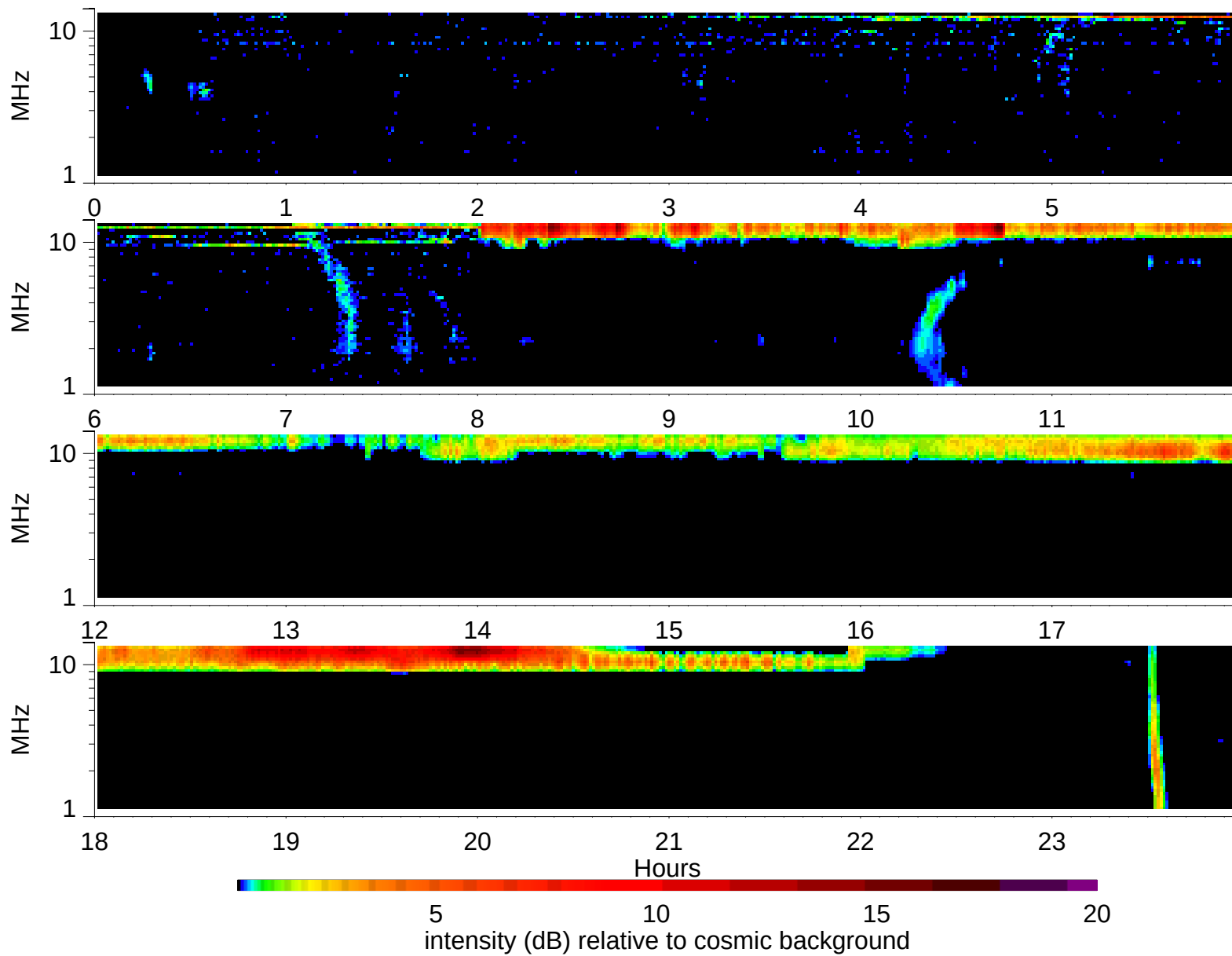
Wind Waves RAD2 receiver: 1995/4/14
