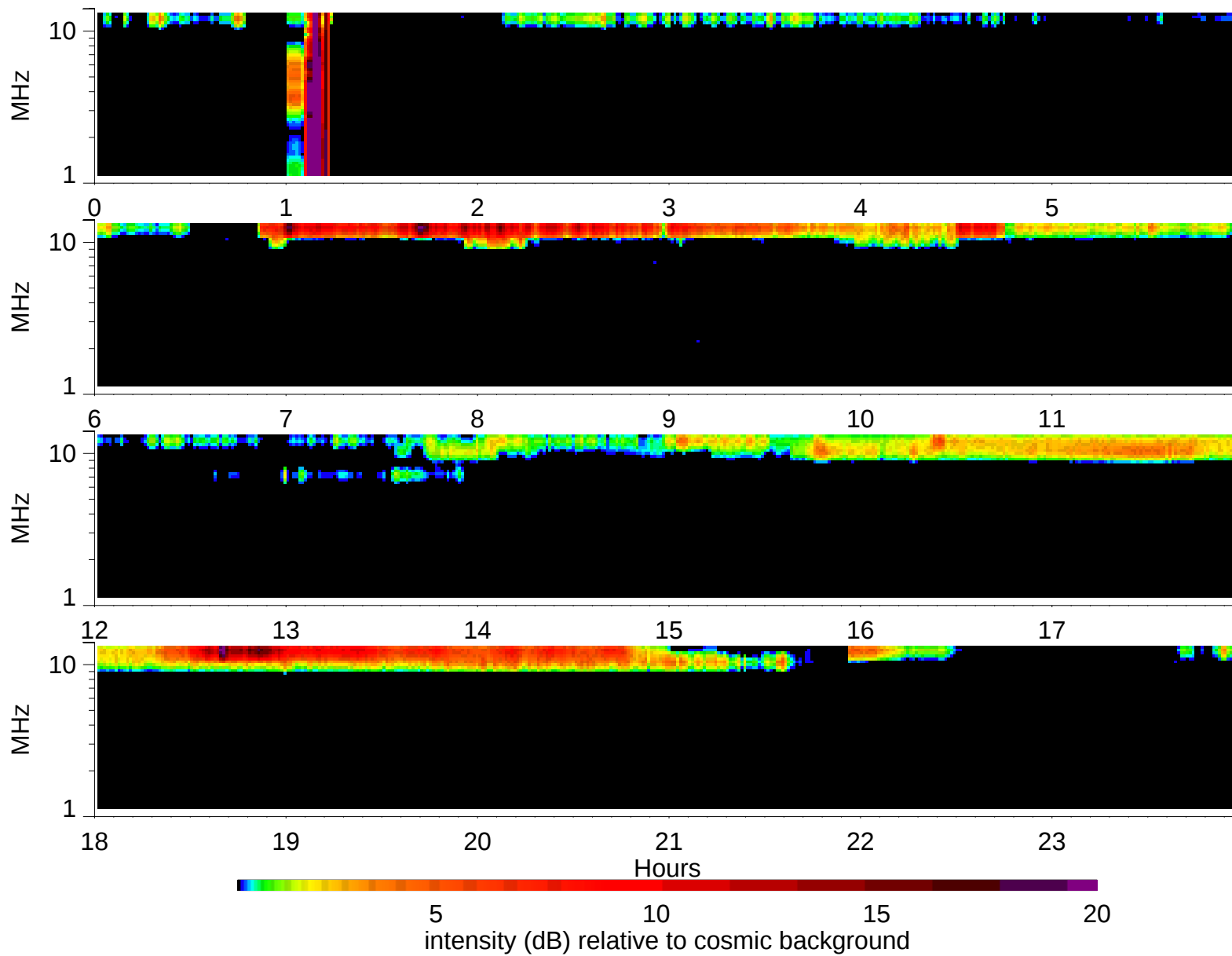
Wind Waves RAD2 receiver: 1995/4/18
