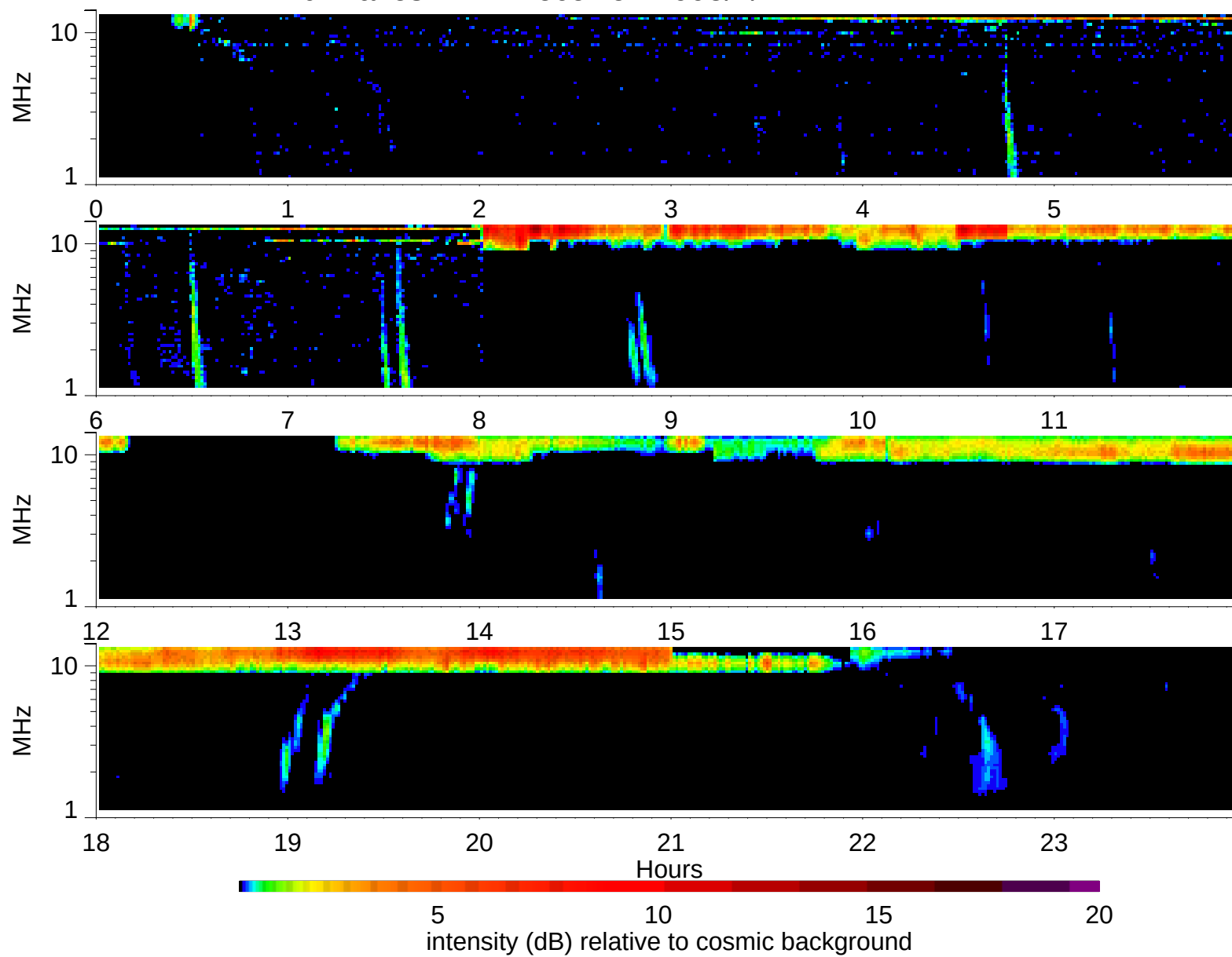
Wind Waves RAD2 receiver: 1995/4/21
