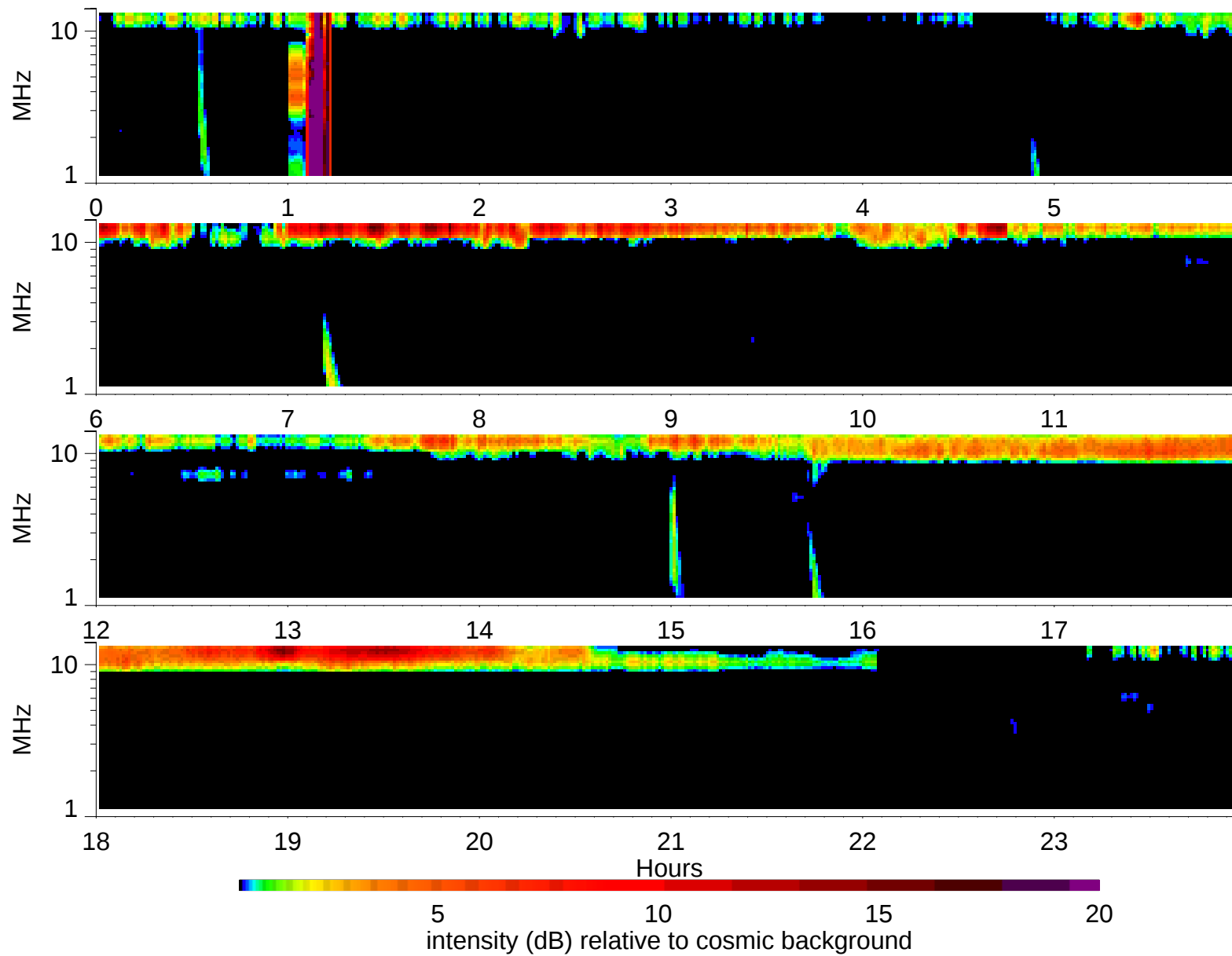
Wind Waves RAD2 receiver: 1995/4/25
