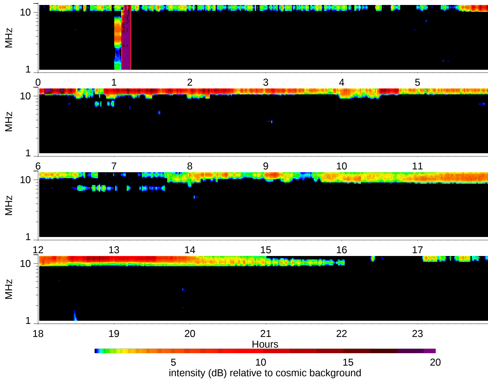
Wind Waves RAD2 receiver: 1995/4/26
