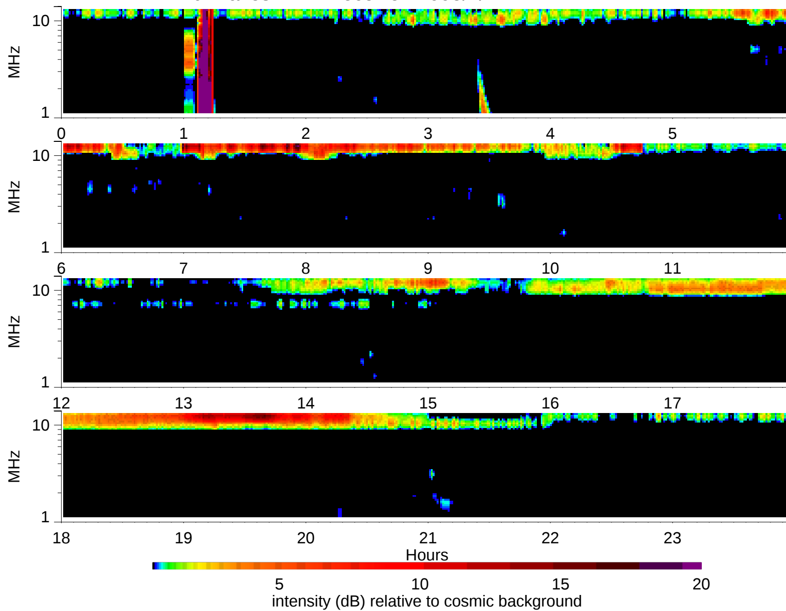
Wind Waves RAD2 receiver: 1995/4/27
