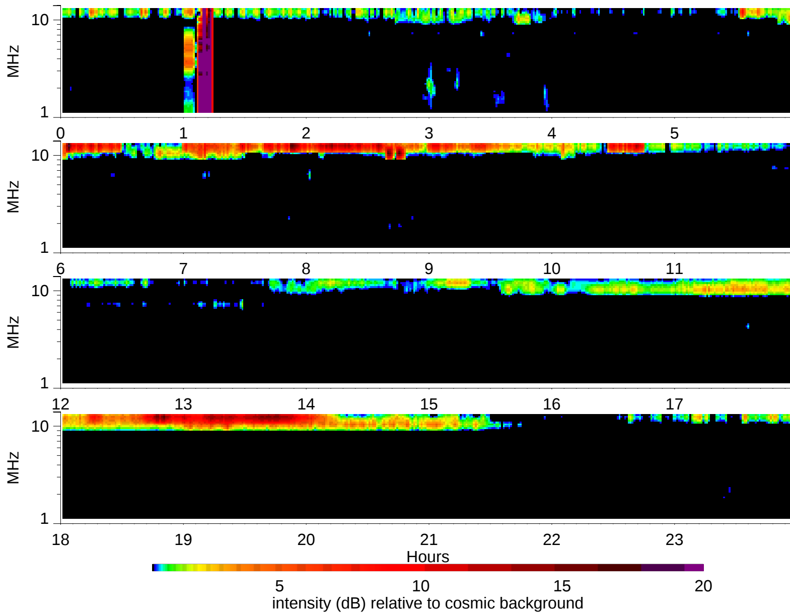
Wind Waves RAD2 receiver: 1995/4/29
