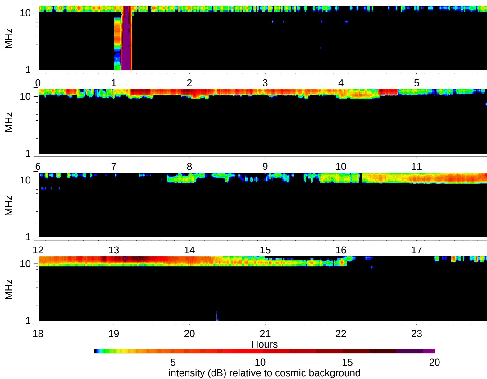
Wind Waves RAD2 receiver: 1995/5/1
