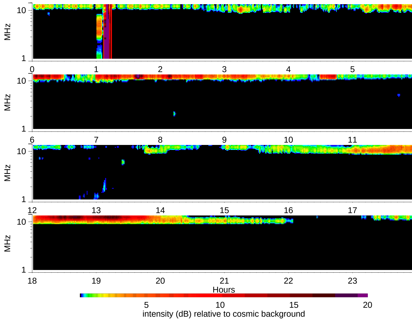
Wind Waves RAD2 receiver: 1995/5/6
