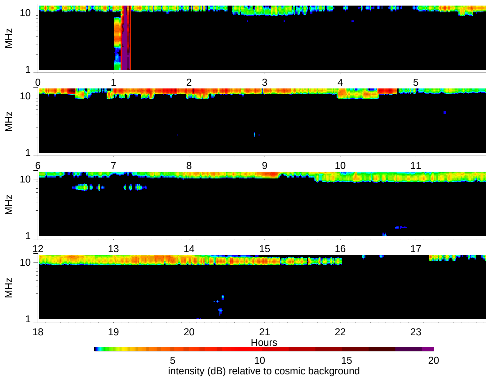
Wind Waves RAD2 receiver: 1995/5/10
