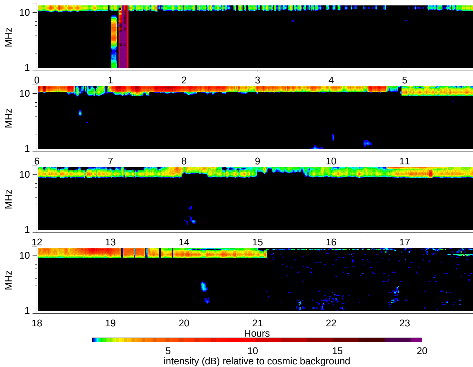
Wind Waves RAD2 receiver: 1995/5/14
