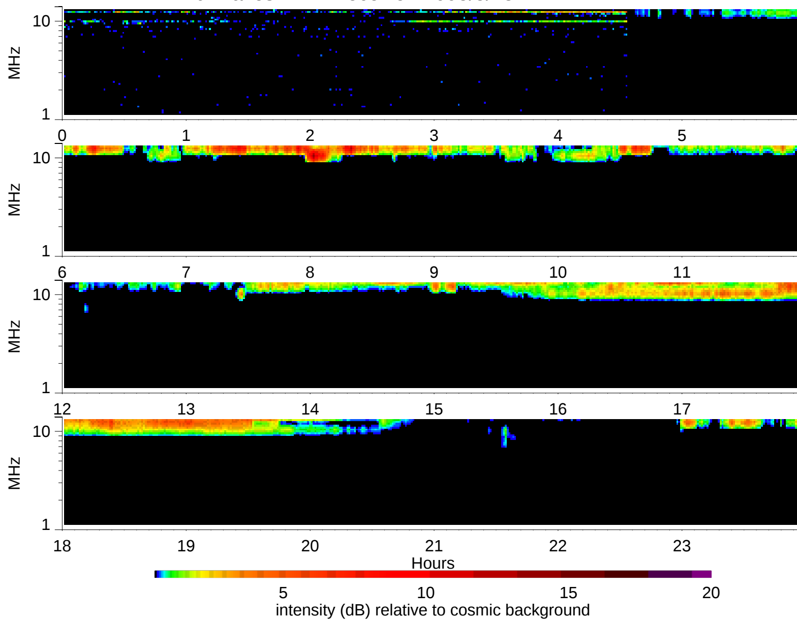
Wind Waves RAD2 receiver: 1995/5/23
