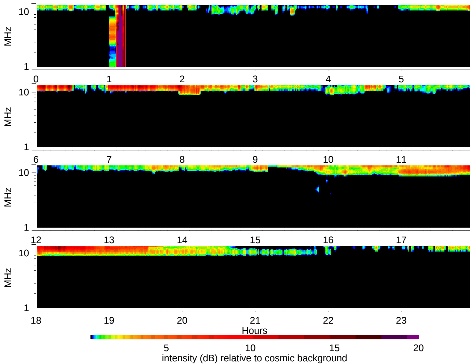
Wind Waves RAD2 receiver: 1995/5/26
