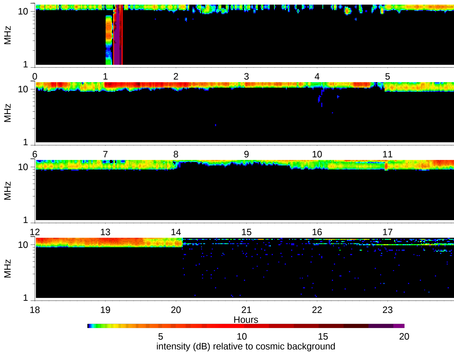
Wind Waves RAD2 receiver: 1995/5/28
