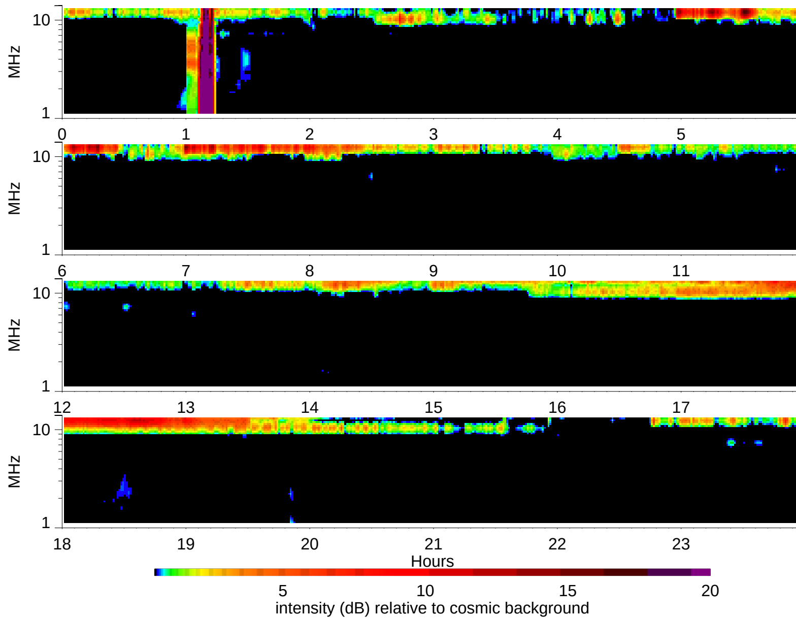
Wind Waves RAD2 receiver: 1995/6/1
