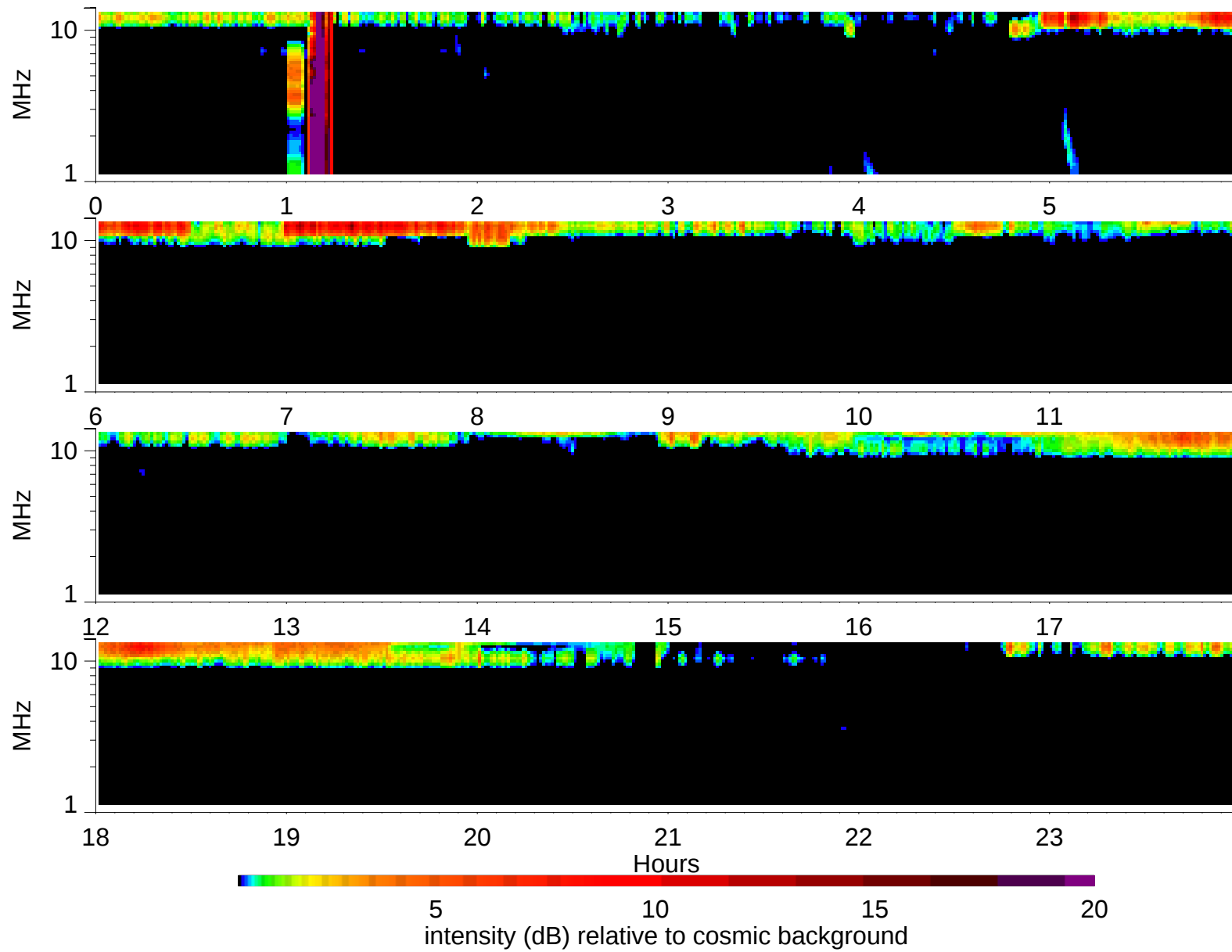
Wind Waves RAD2 receiver: 1995/6/5
