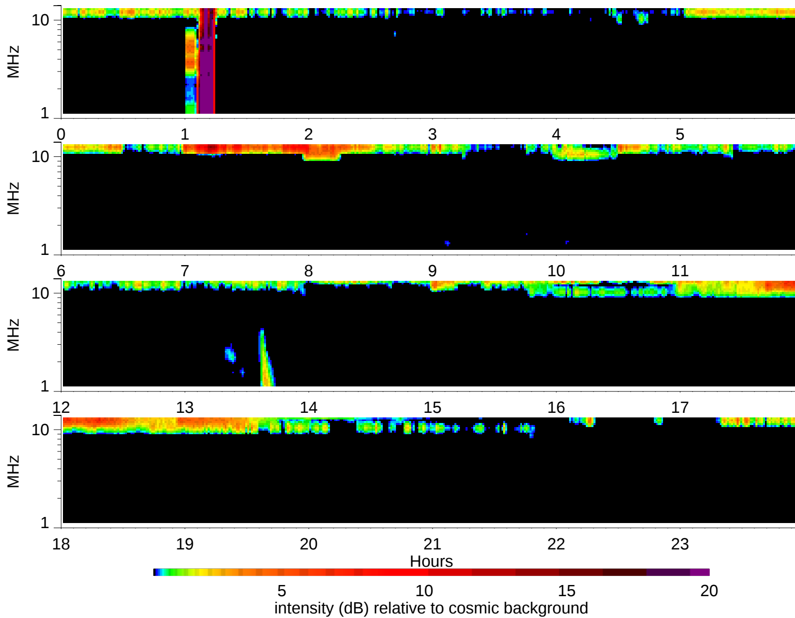
Wind Waves RAD2 receiver: 1995/6/7
