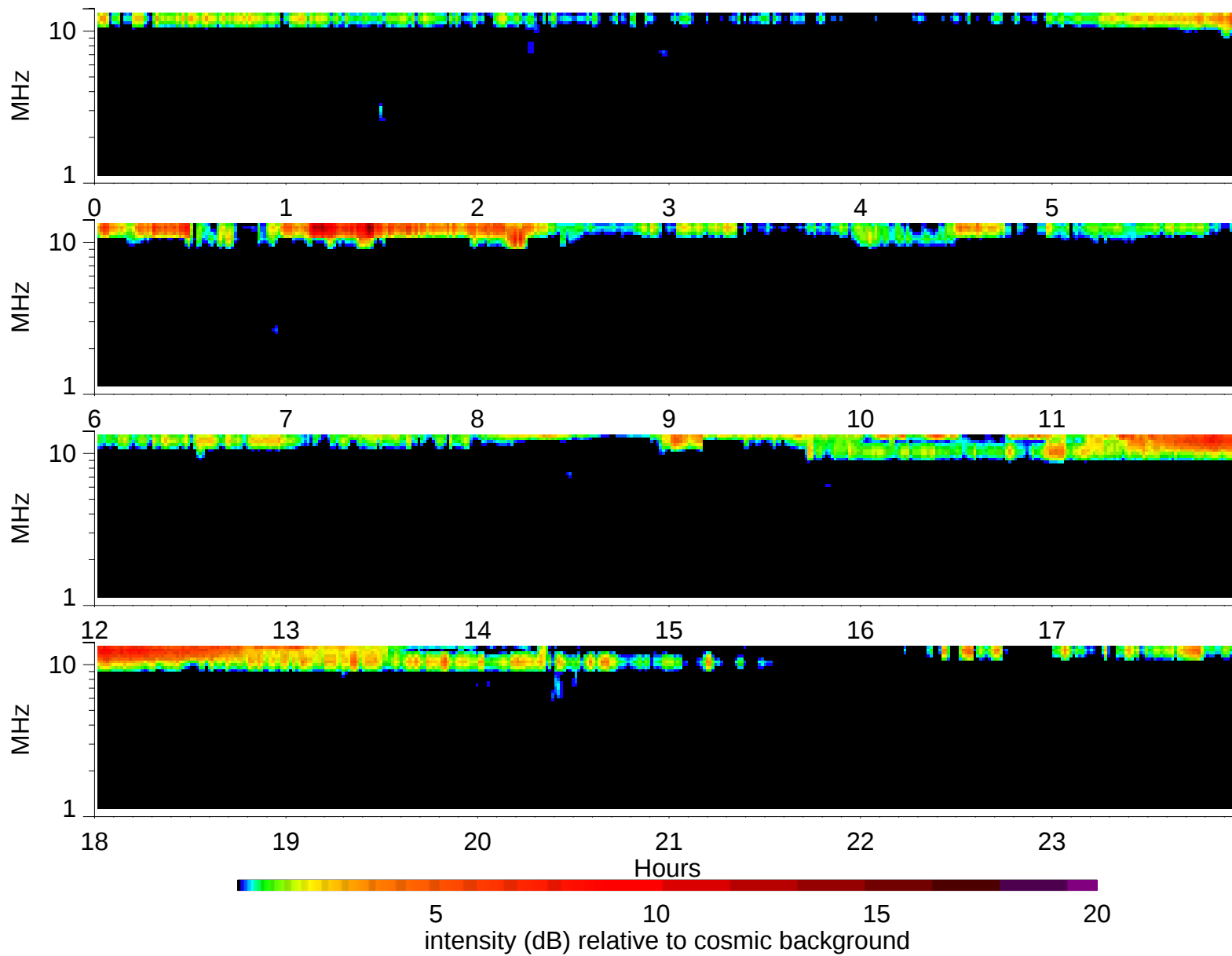
Wind Waves RAD2 receiver: 1995/6/8
