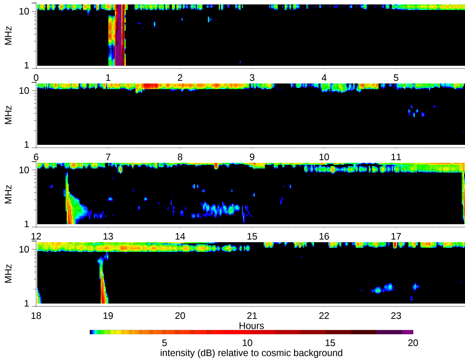
Wind Waves RAD2 receiver: 1995/6/9
